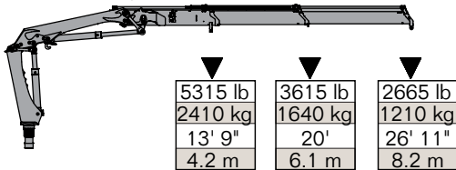
11/78DL - 2 Hydraulic
