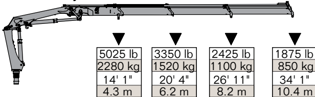
11/78DL - 3 Hydraulic
