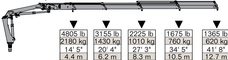
11/78DL - 4 Hydraulic
