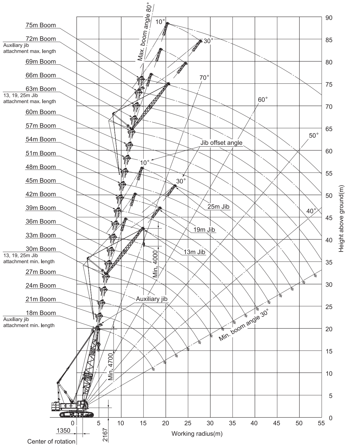
Main boom + Auxiliary jib
