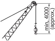
Auxiliary jib
