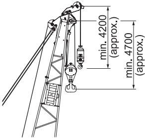
Main boom + Auxiliary jib
