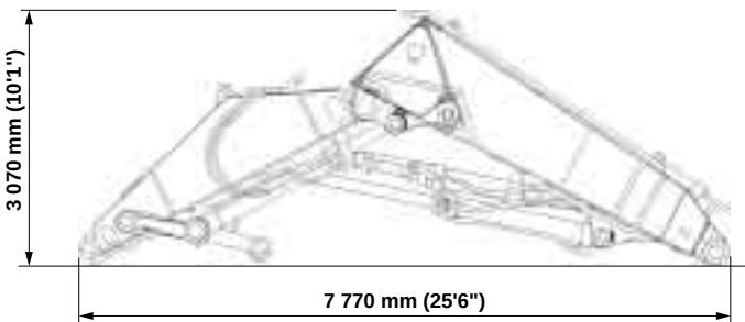
Loading Shovel Front Attachment (Without Bucket)
