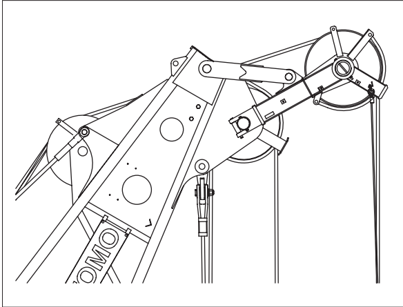
Auxiliary short jib (Option)
