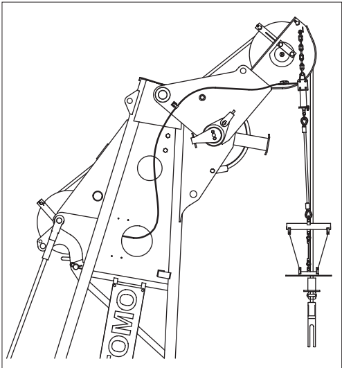
Short jib (Option)
