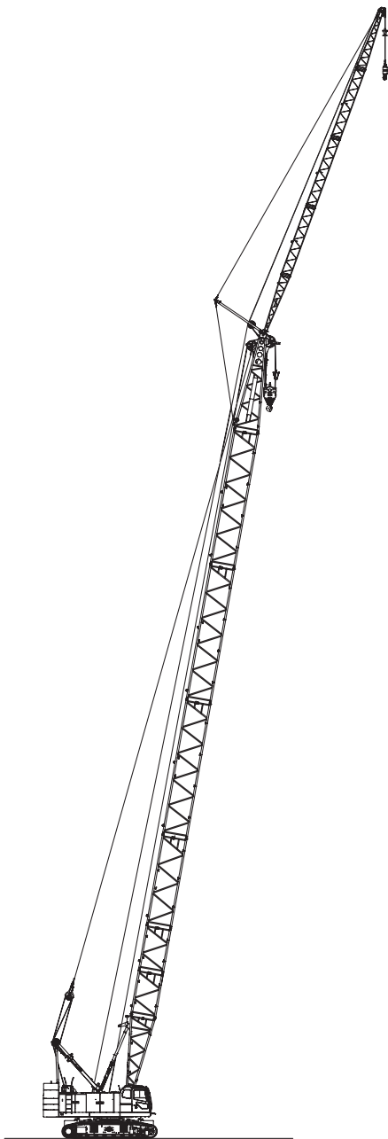
Crane Specification (Boom Longest Length with Crane Jib)
