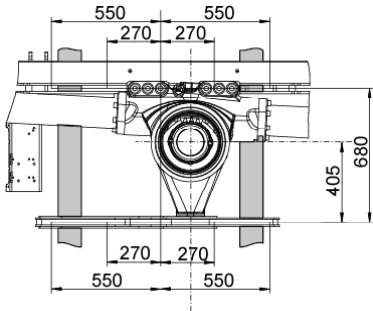
Chassis Installation
