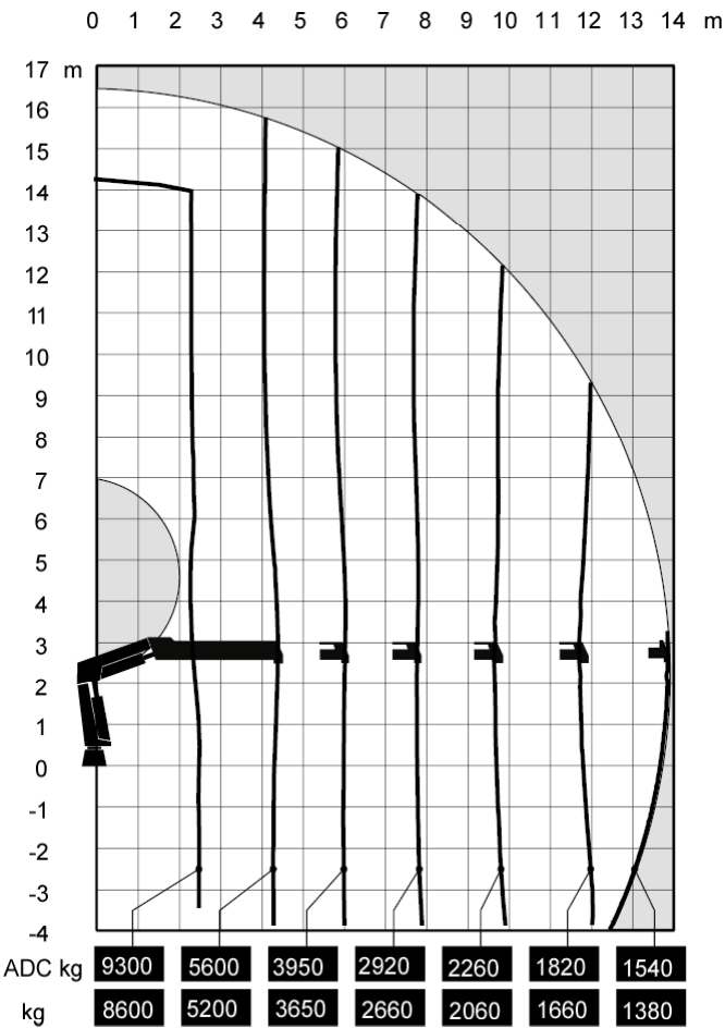
Load Diagram
