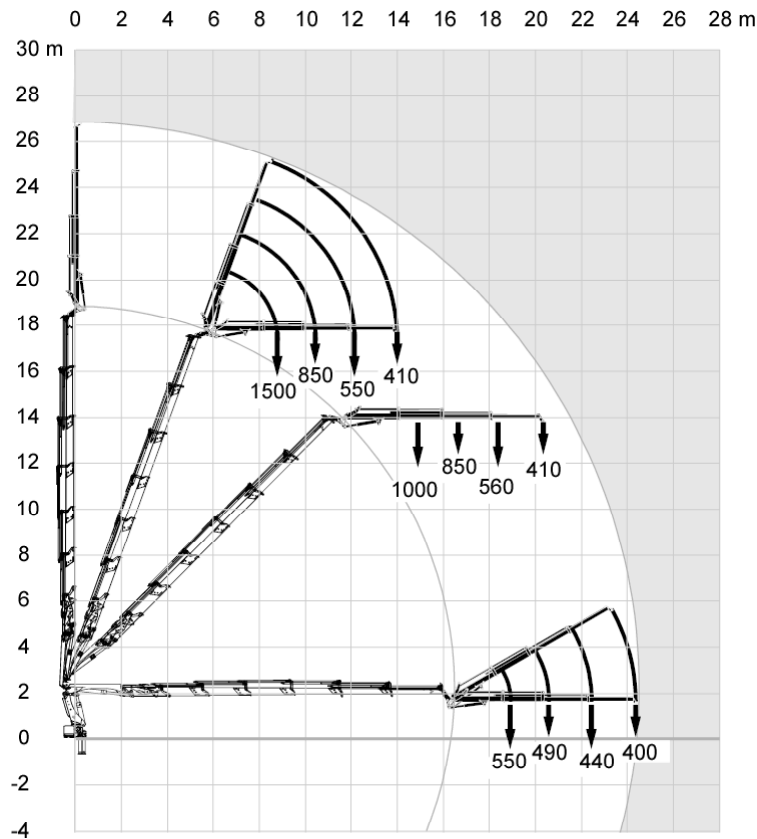
Load Diagram
