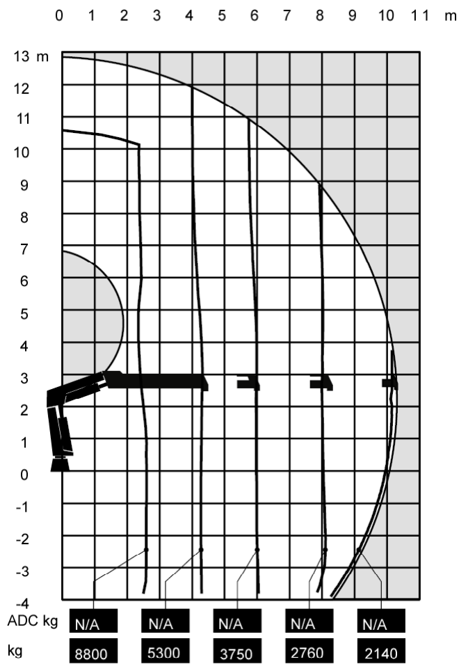
Load Diagram
