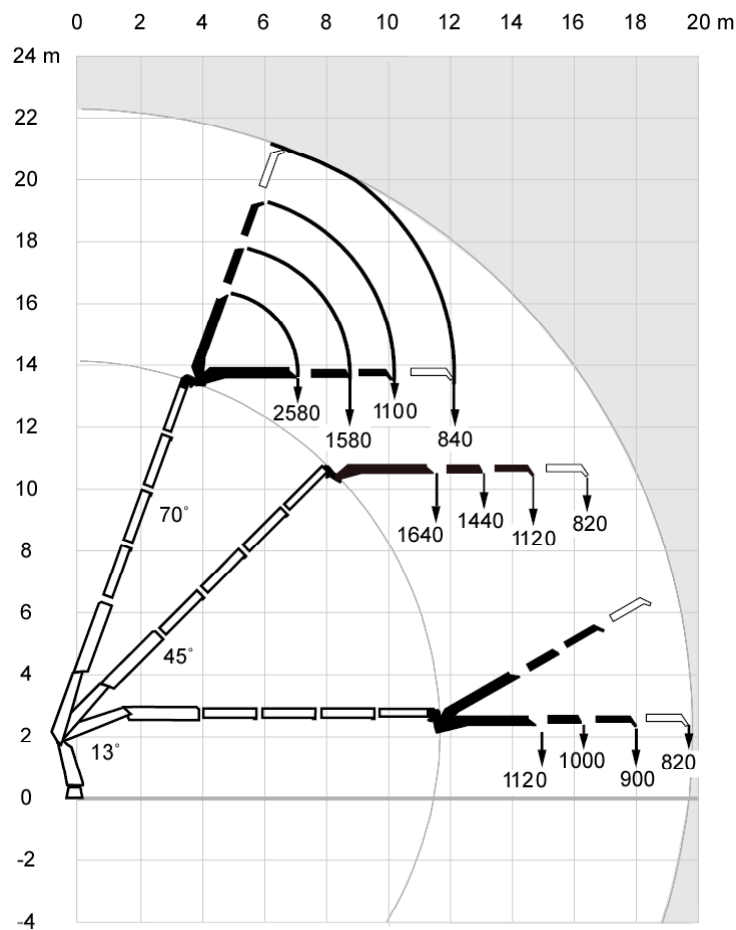
Load Diagram
