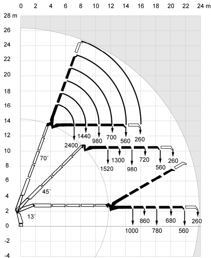
Load Diagram
