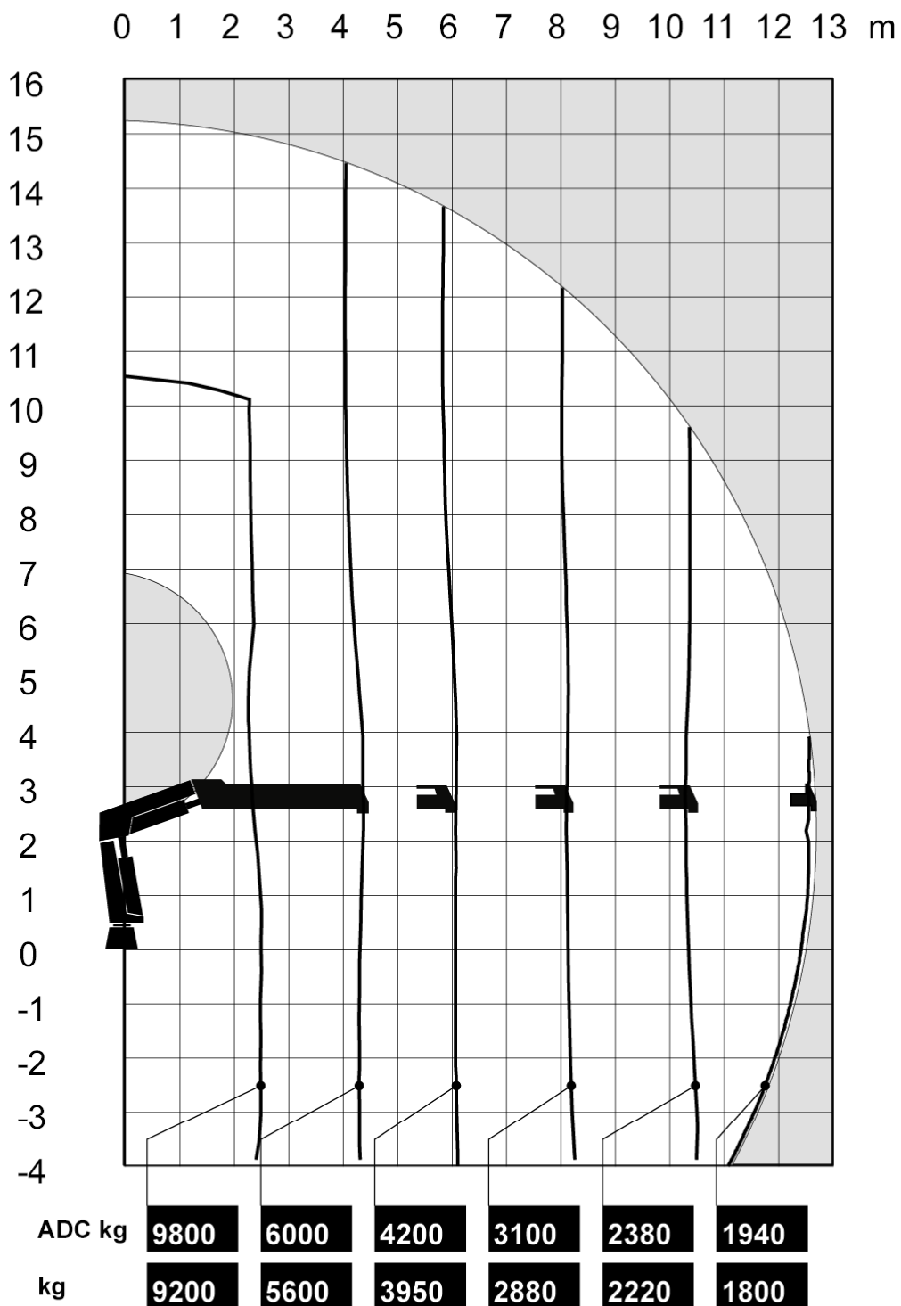
Load diagram
