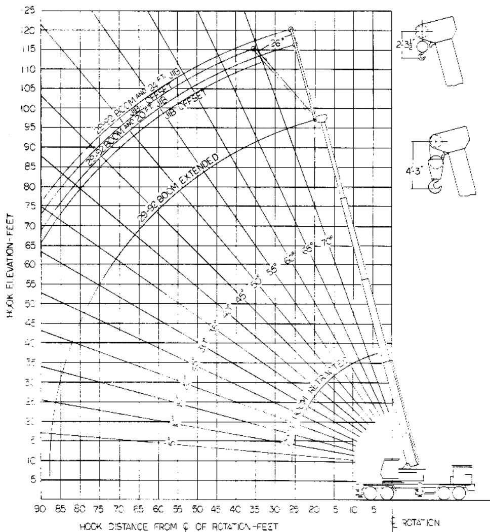
RATED LIFTING CAPACITIES, 29' - 92' FOUR SECTION BOOM OVER SIDE AND REAR ON OUTRIGGERS
