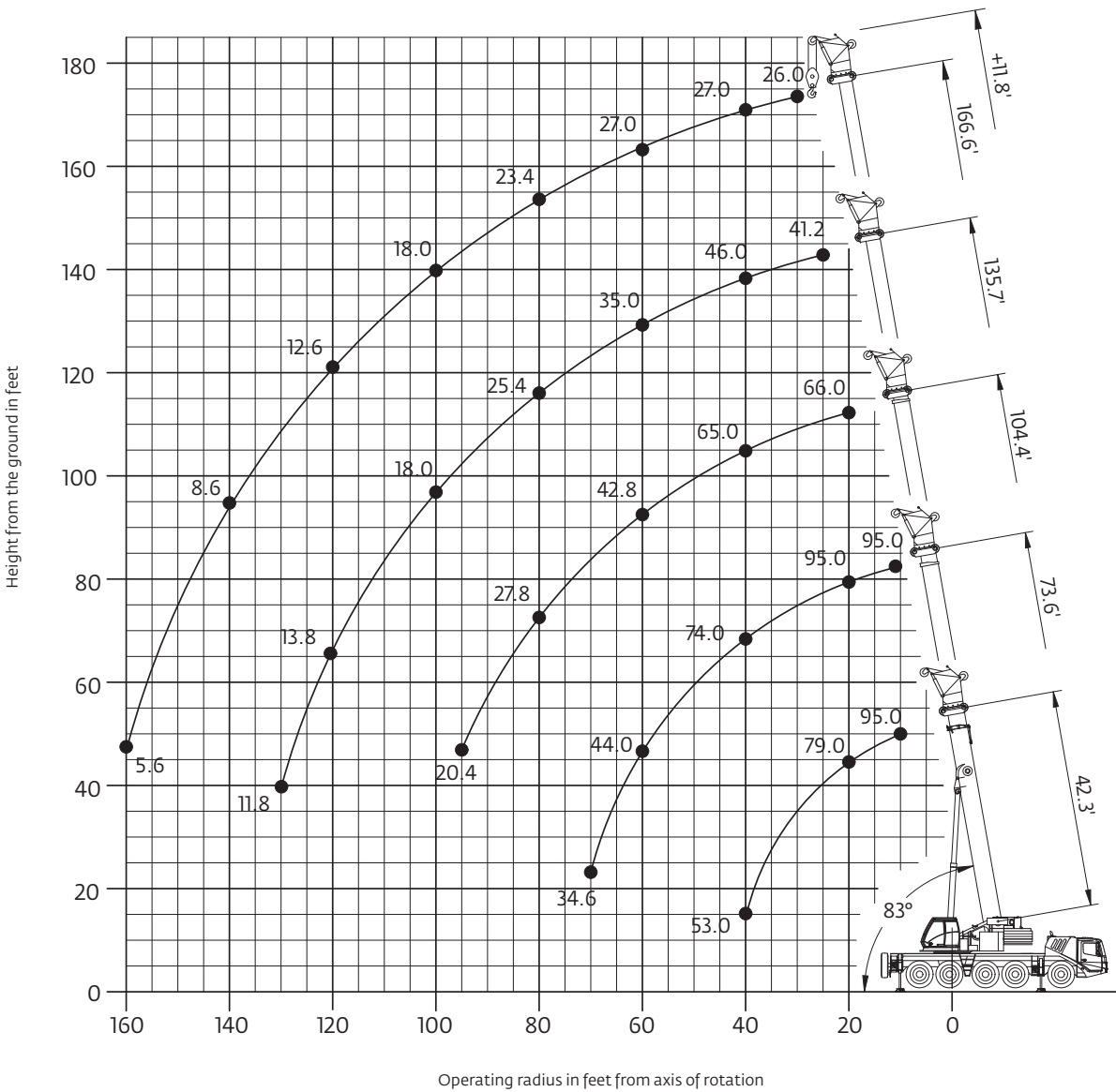
42 ft – 167 ft main boom with 12 ft integrated heavy duty jib
