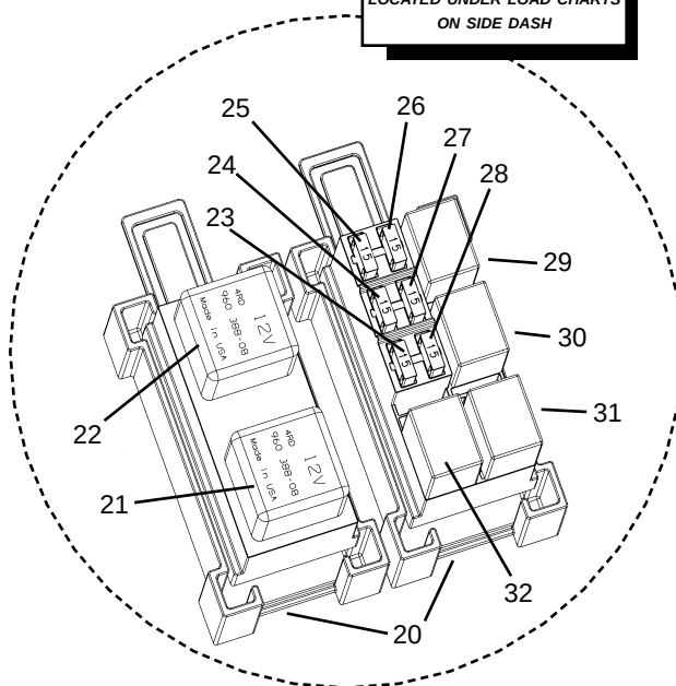
FUSES AND RELAYS LOCATED UNDER LOAD CHARTS ON SIDE DASH
