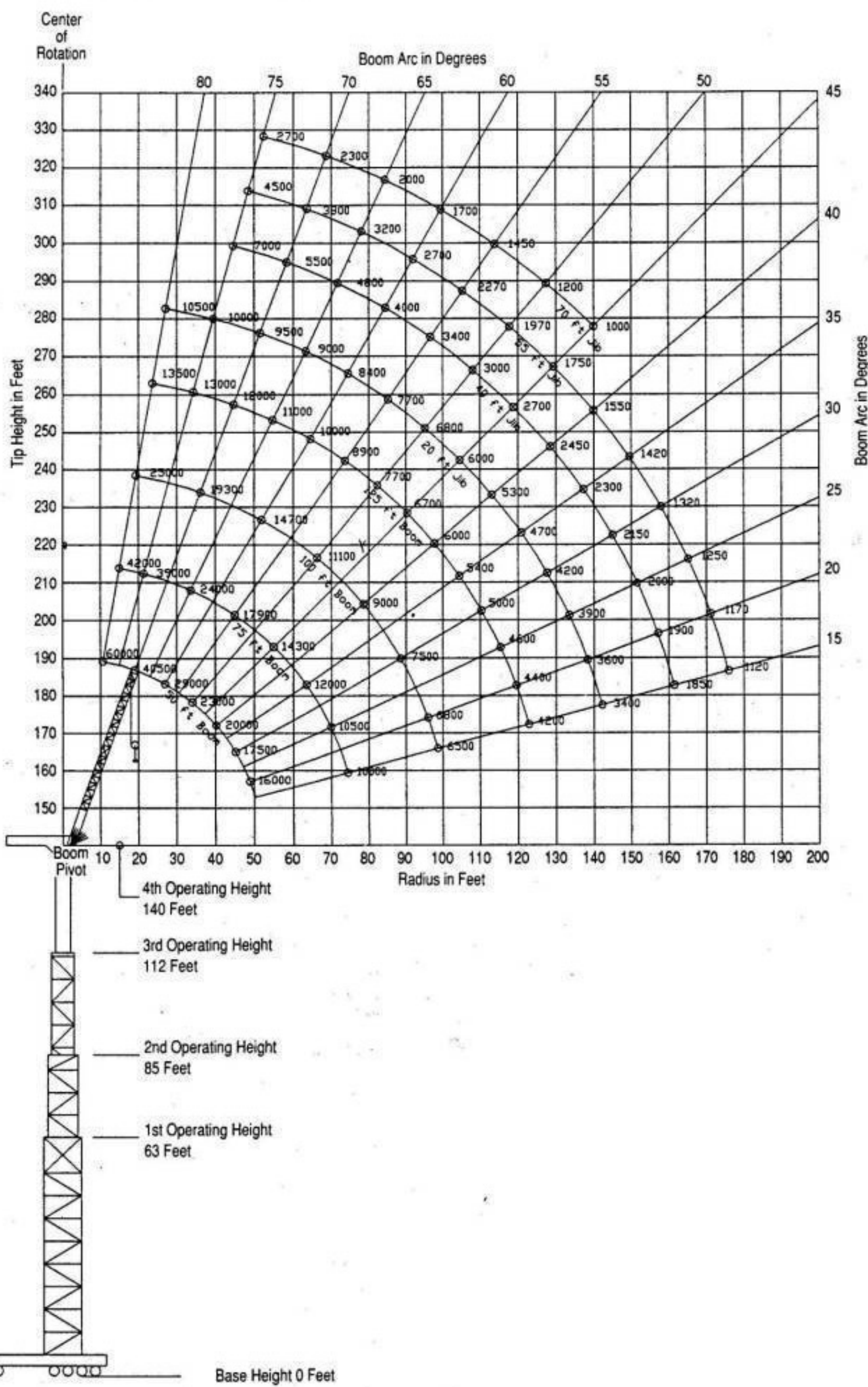
GCI LATTICE BOOM RATED LIFTING CAPACITY
