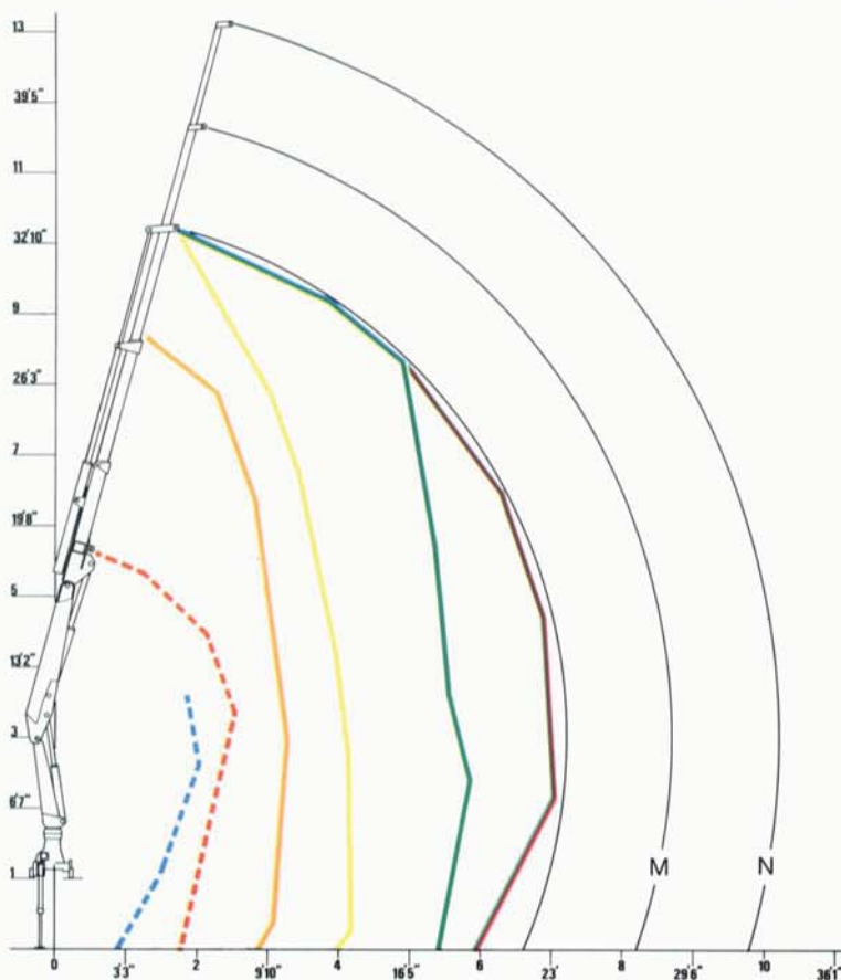
CAPACITY CHART - diagram hefvermogen DIAGRAMA DE CARGA
