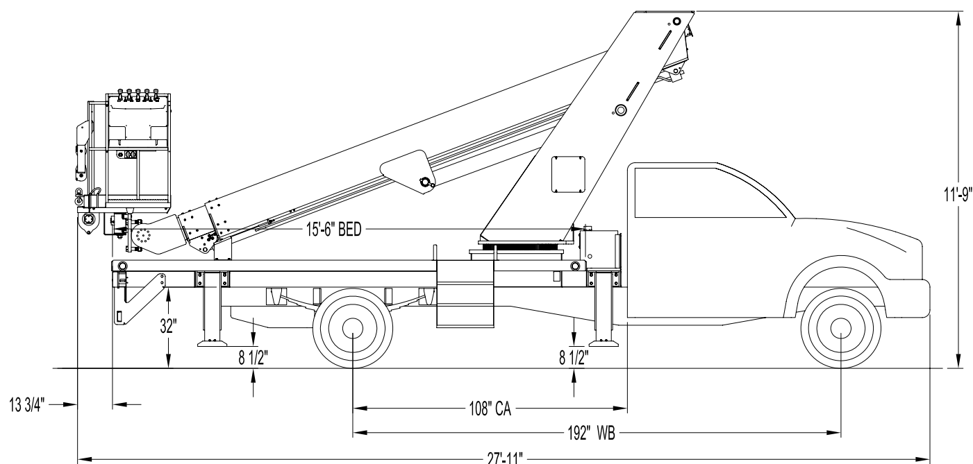
V60F SIDE VIEW DIAGRAM
