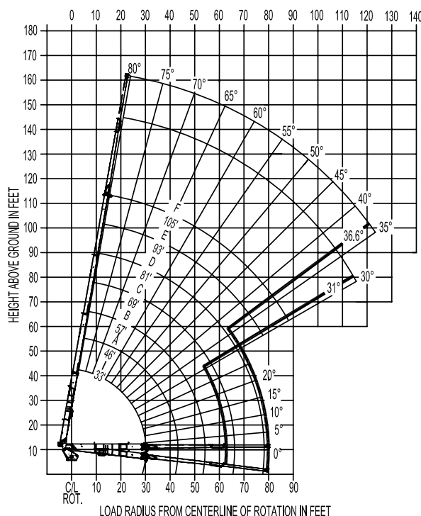
JIB RANGE DIAGRAM WITH FULL SPAN OUTRIGGERS
