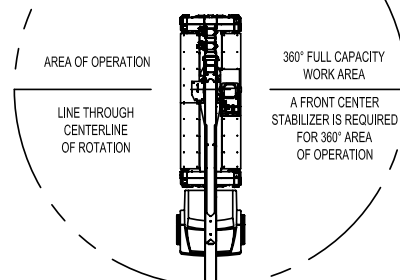
NO-SPAN OUTRIGGERS HORIZONTAL BEAMS FULLY RETRACTED VERTICAL CYLINDERS STRAIGHT DOWN
