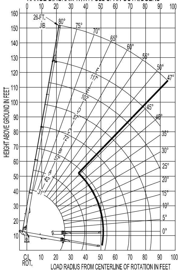
PRELIMINARY RANGE DIAGRAM WITH FULL SPAN OUTRIGGERS
