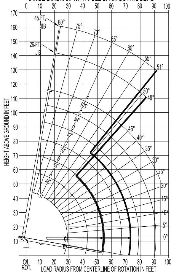
PRELIMINARY RANGE DIAGRAM WITH FULL SPAN OUTRIGGERS
