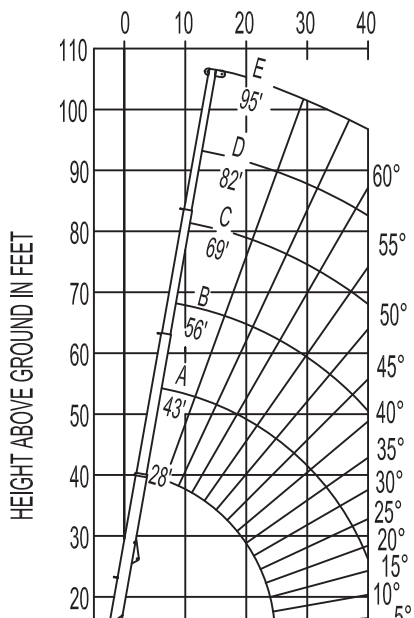
RANGE DIAGRAM WITH OUTRIGGERS AT FULL HORIZONTAL RETRACTED POSITION
