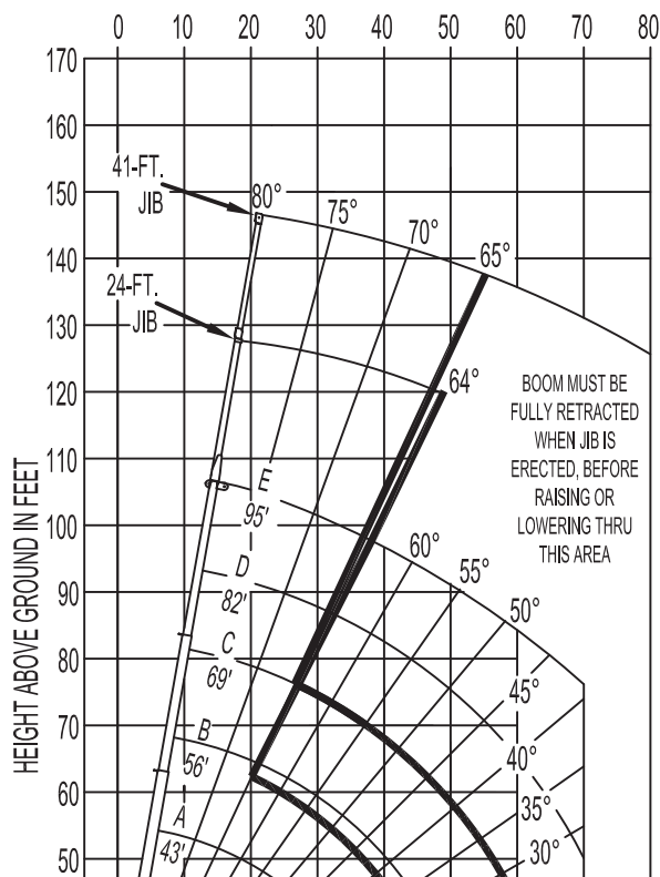
RANGE DIAGRAM WITH OUTRIGGERS AT MID-SPAN POSITION
