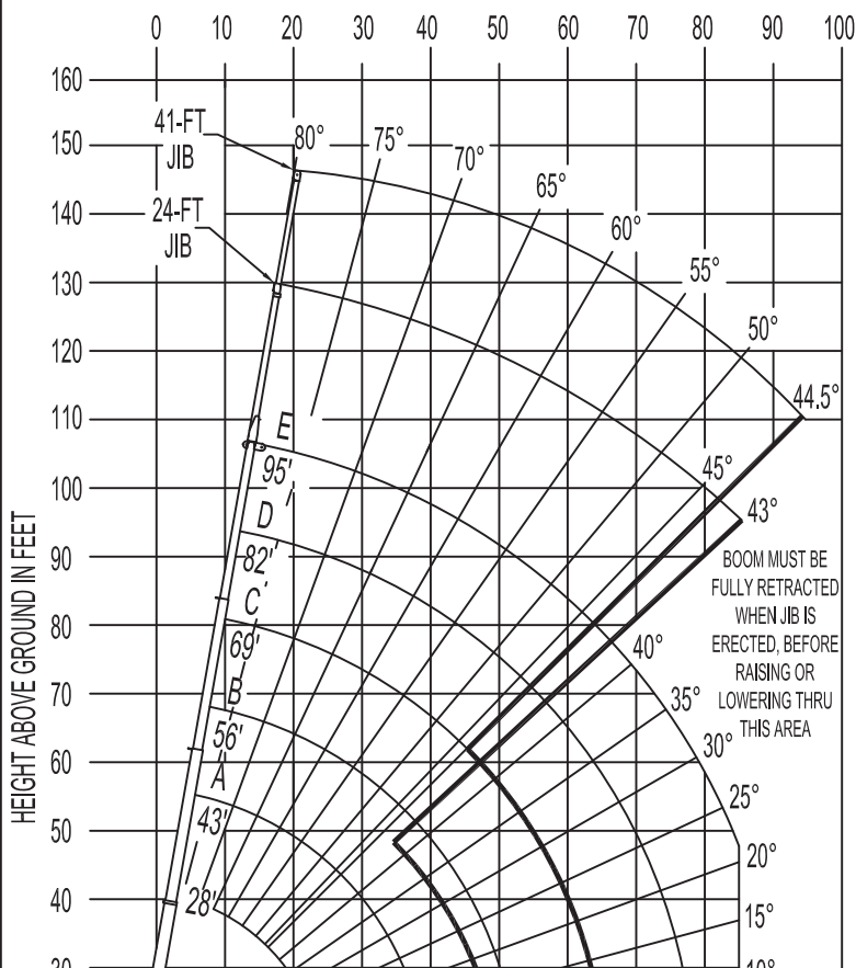
RANGE DIAGRAM WITH FULL SPAN OUTRIGGERS
