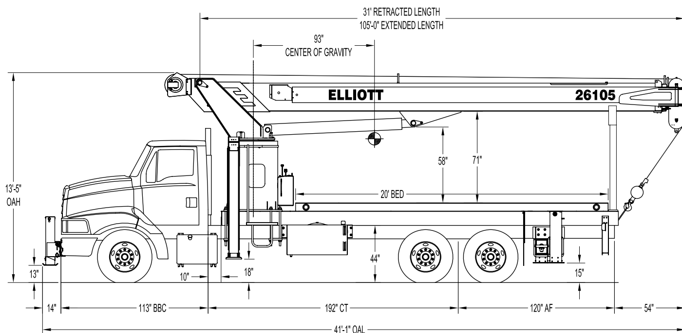
26105F SIDE VIEW DIAGRAM
