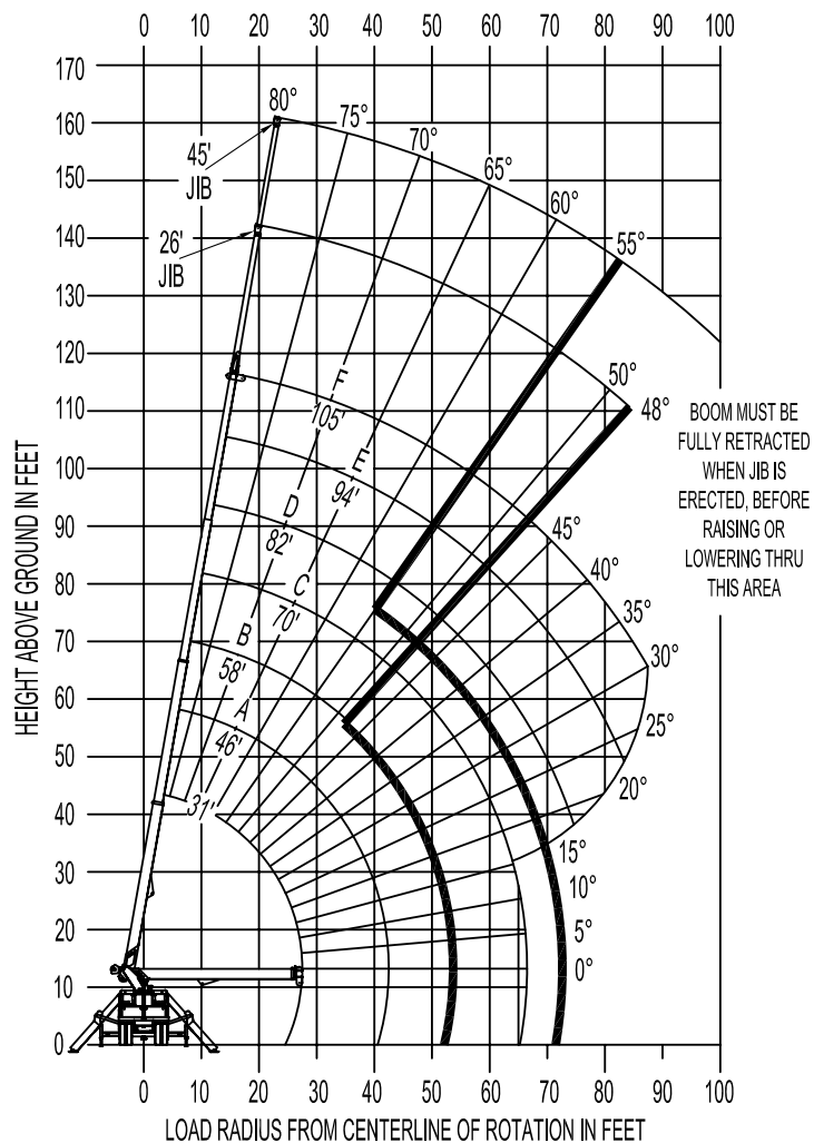
RANGE DIAGRAM WITH FULL SPAN OUTRIGGERS
