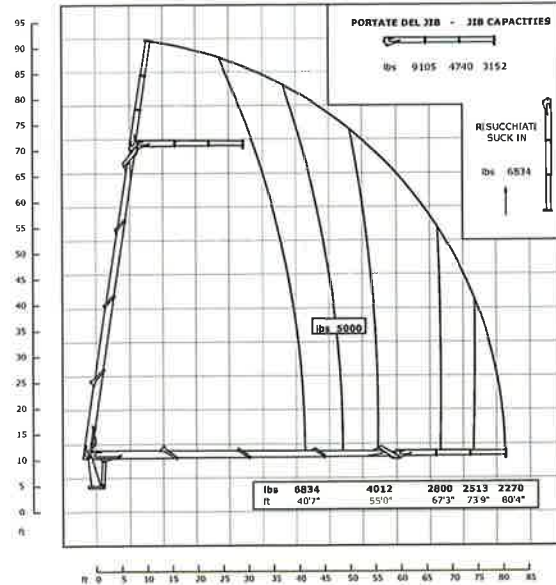
50000 WB87
