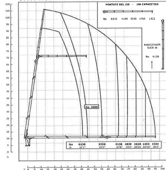
50000 WB95
