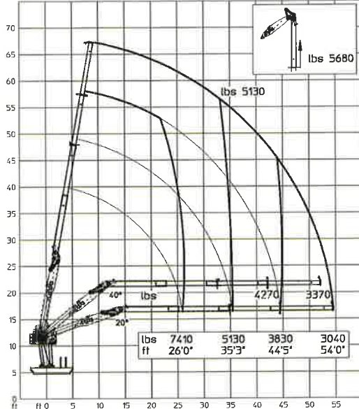
30000 WB65
