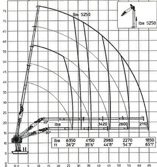
30000 WB65
