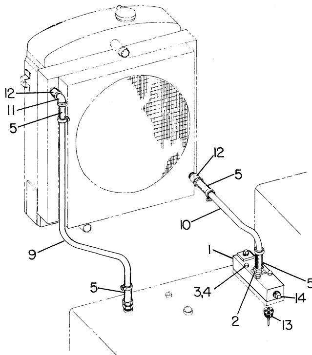
BEGINNING W/SER. #390
