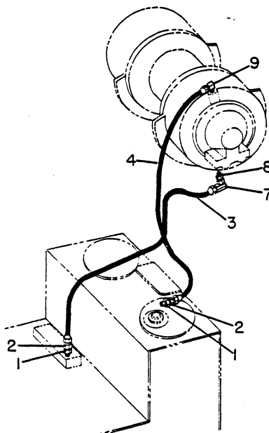
MODEL 22 WINCH
