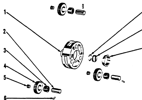
FIGURE 2 - MODEL 11E
