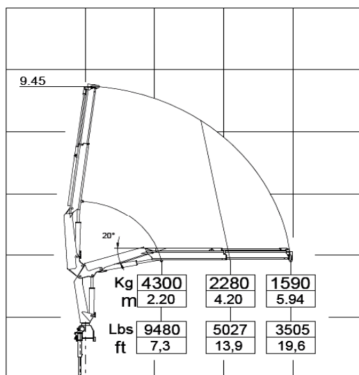
AC10-69 1 Hydraulic Extension
