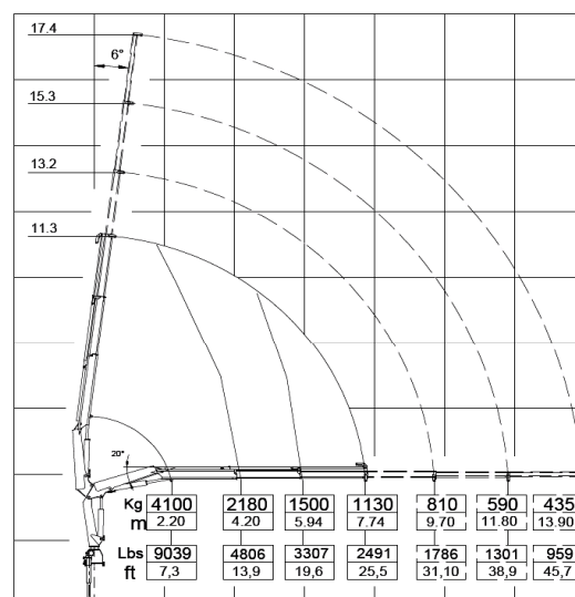
AC10-69 2 Hydraulic Extension
