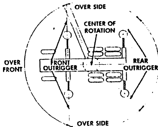
DIAGRAM NO. 2 OUTRIGGERS EXTENDED & SET
