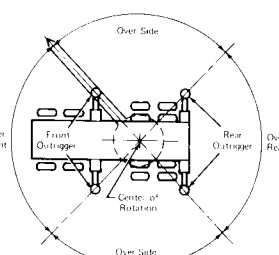
DIAGRAM NO. 2 OUTRIGGERS EXTENDED AND SET
