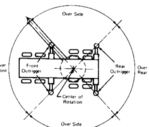
DIAGRAM NO. 2 OUTRIGGERS EXTENDED AND SET
