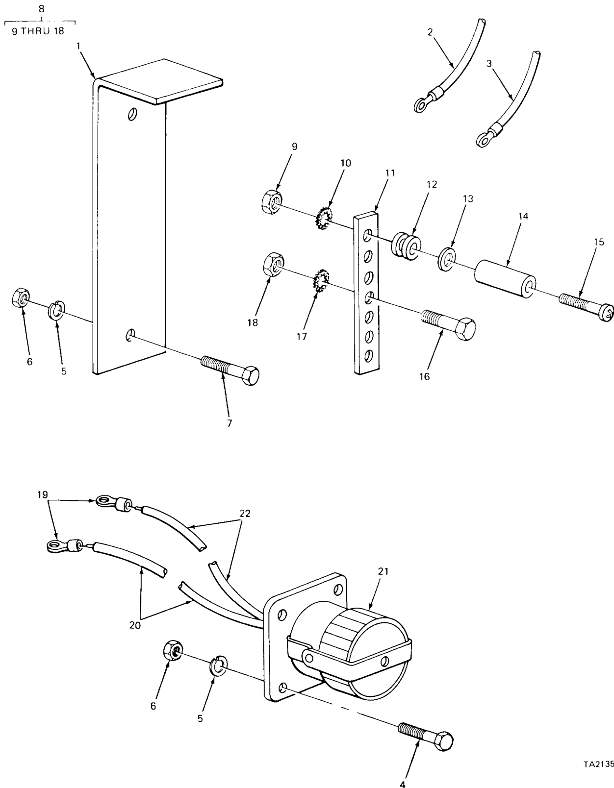
FIGURE 87. BUS BAR AND RECEPTACLE (CRANE).
