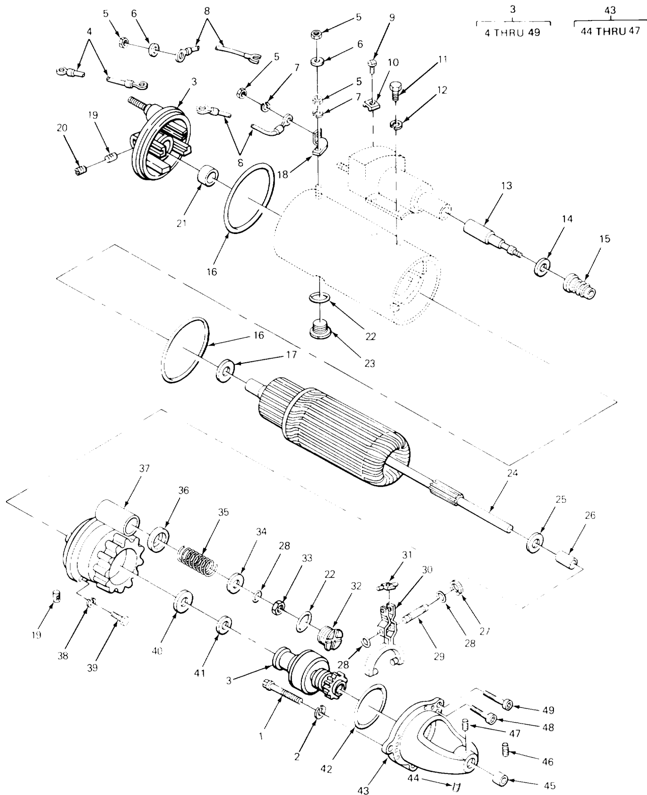
FIGURE 77. STARTER ASSEMBLY
