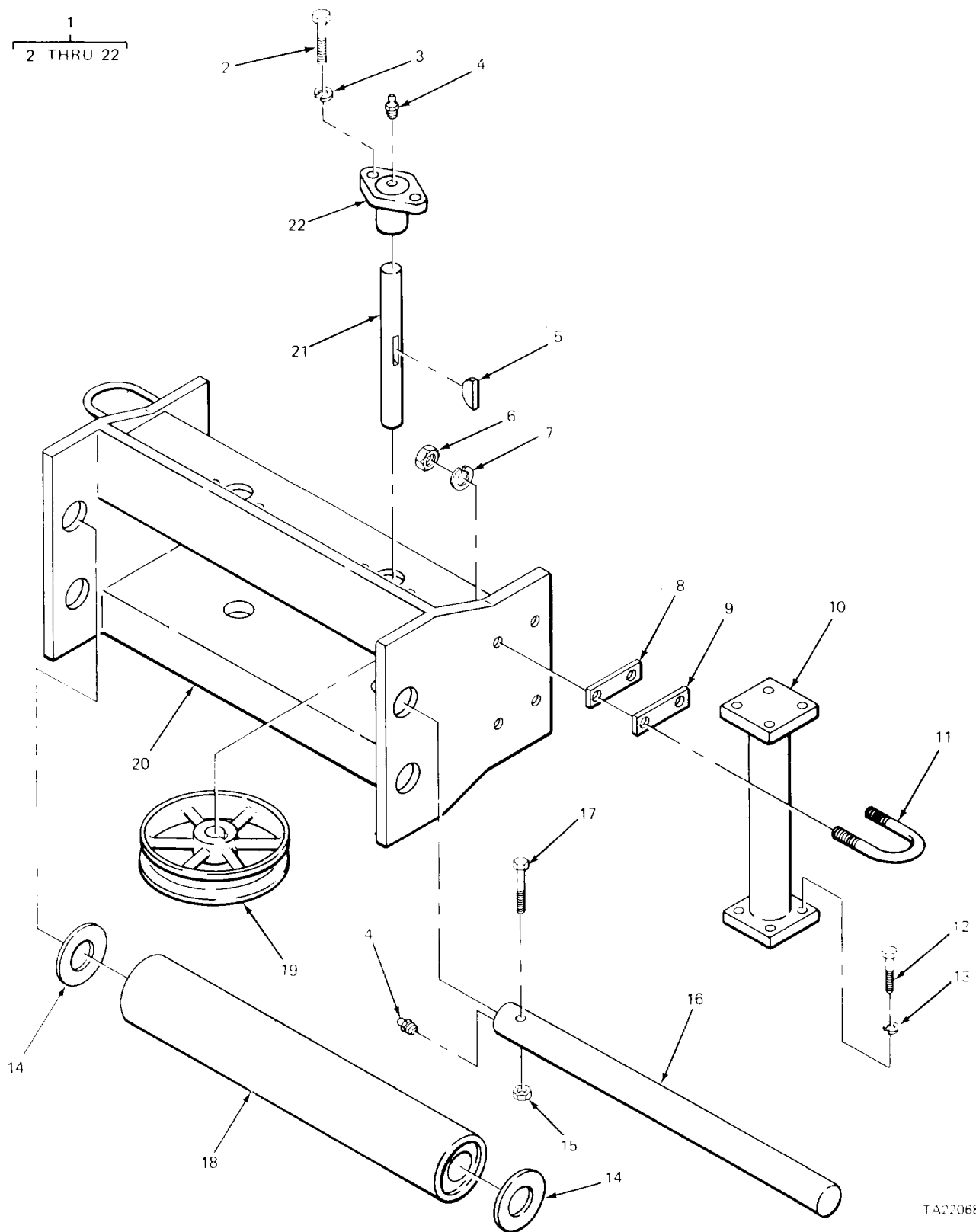
FIGURE 271. FAIR LEAD.
