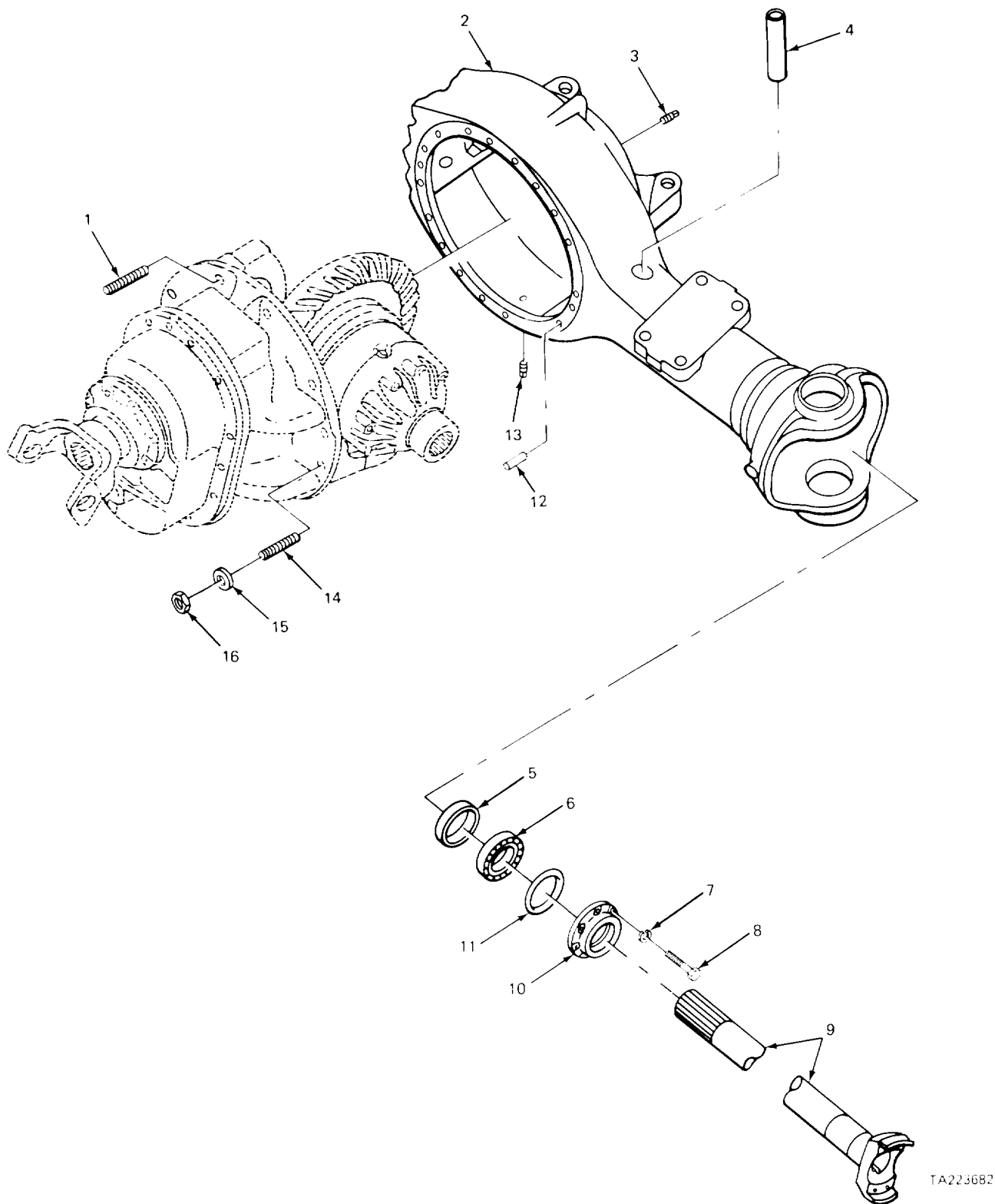
FIGURE 133. REAR AXLE SHAFT AND HOUSING (CARRIER).
