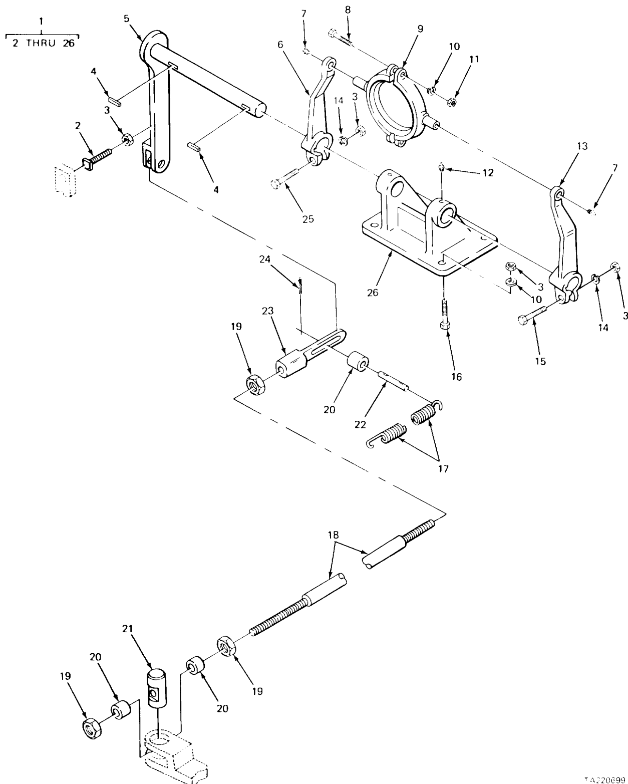
FIGURE 283. INDEPENDENT BOOM HOIST CONTROL.
