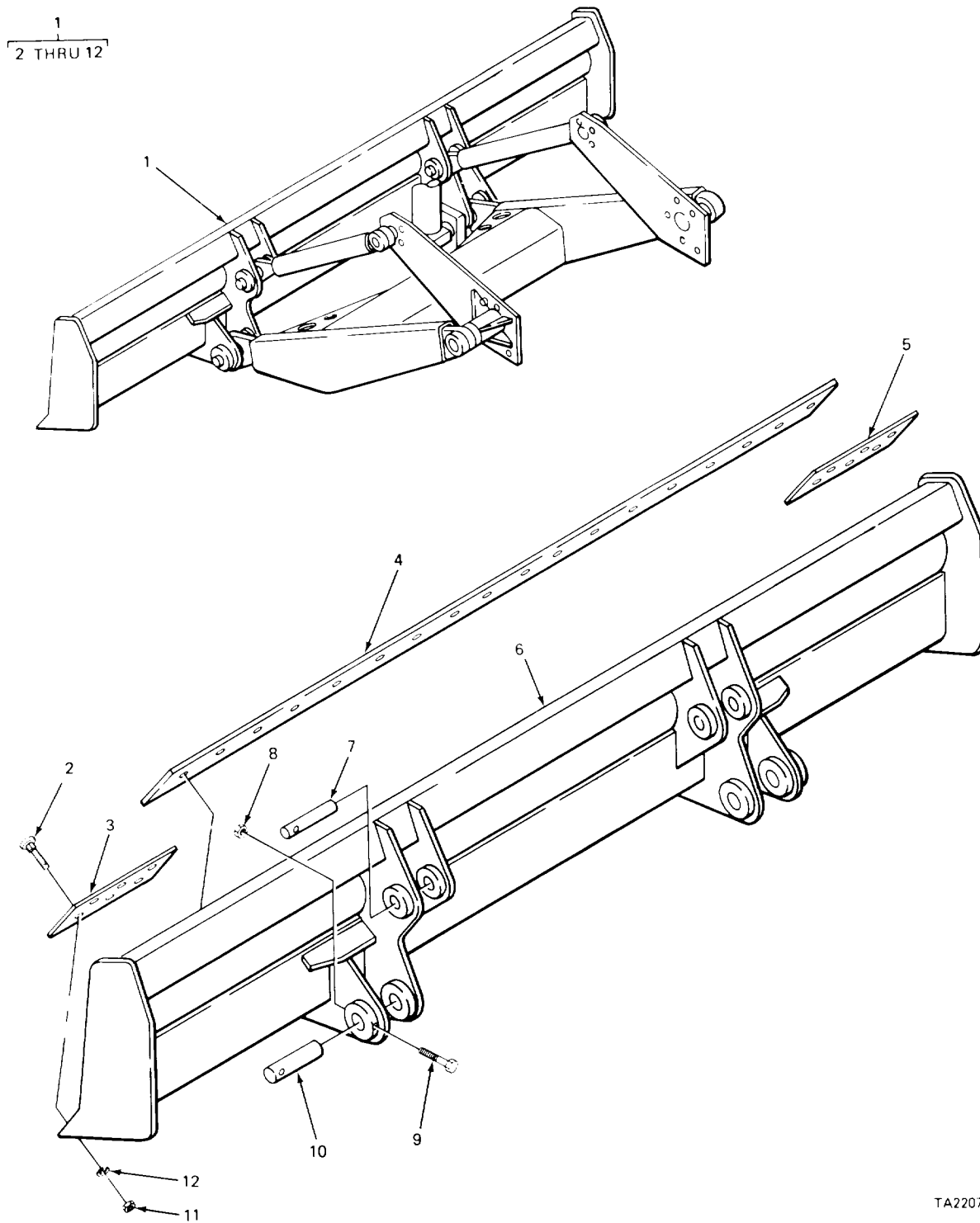
FIGURE 291. UTILITY BLADE ASSEMBLY.
