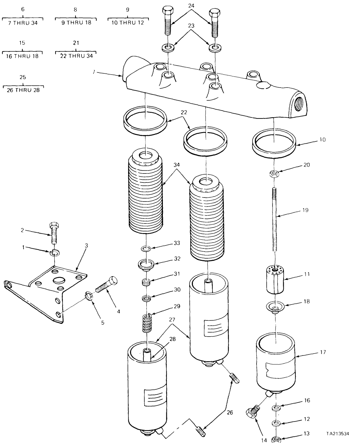
FIGURE 44. FUEL FILTER (CRANE).
