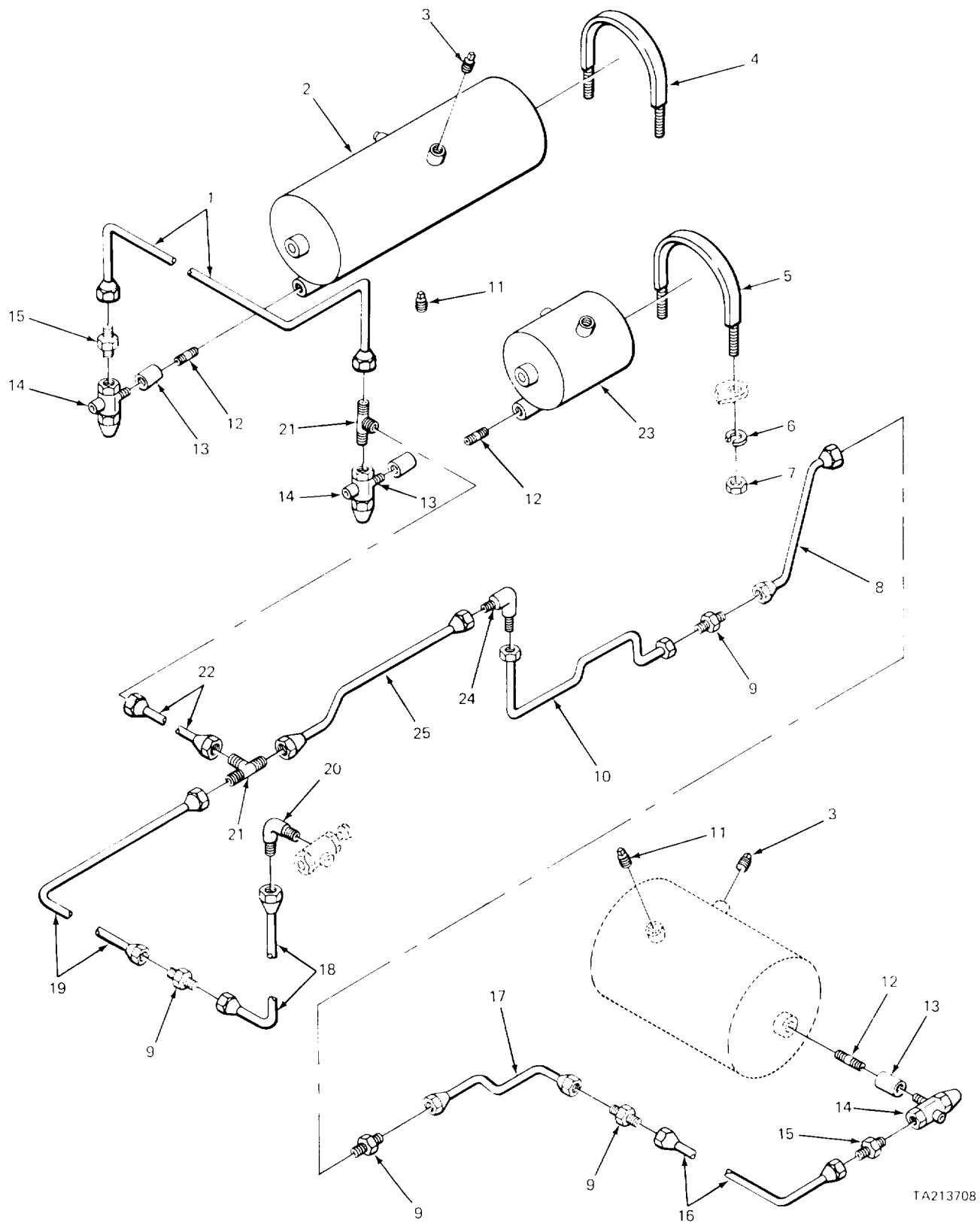
FIGURE 149. AIR RESERVOIR AND AIR LINES (MODEL 2385 CARRIER).
