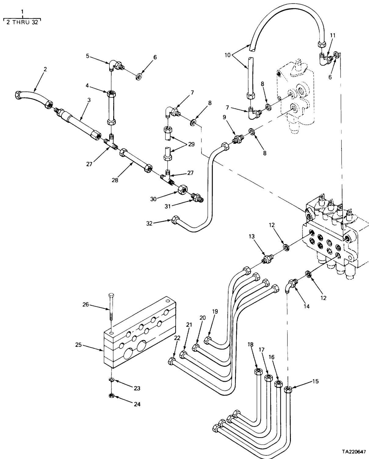
FIGURE 247. CAB HYDRAULIC PIPING (MODEL 2385 CARRIER).
