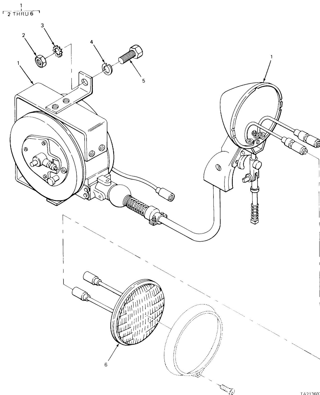
FIGURE 95. TROUBLE LIGHT (CARRIER).
