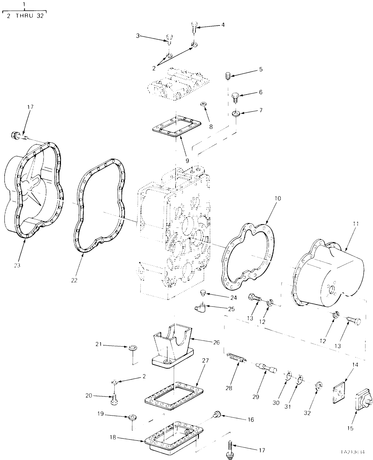
FIGURE 113. TRANSMISSION ASSEMBLY AND COMPONENT PARTS (CARRIER)
