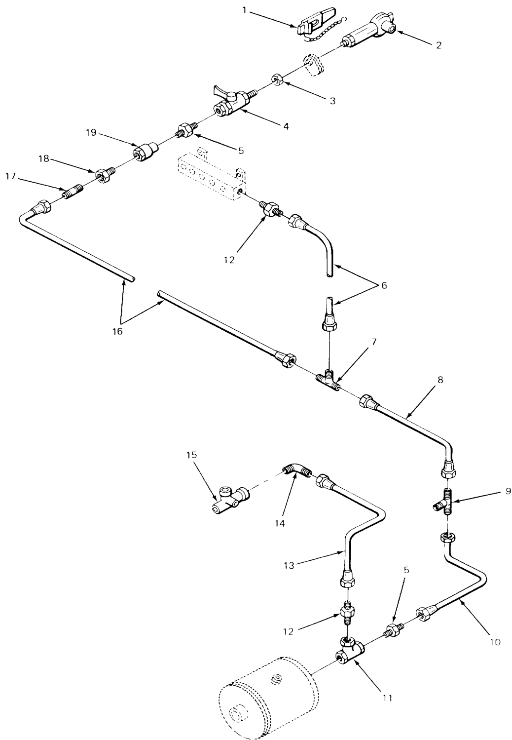
FIGURE 146. AIR BRAKE QUICK DISCONNECT AND RELATED PARTS (MODEL 2385 CARRIER).
