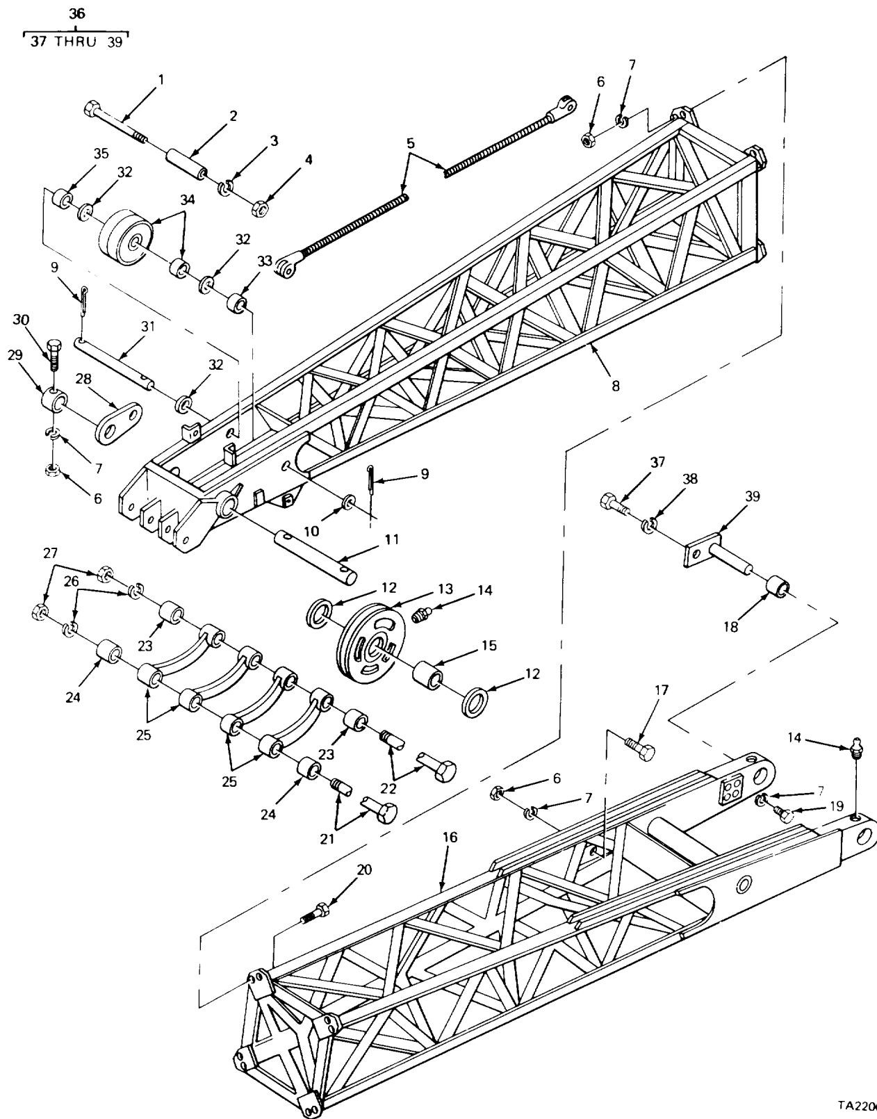
FIGURE 257. BOOM (CRANE).
