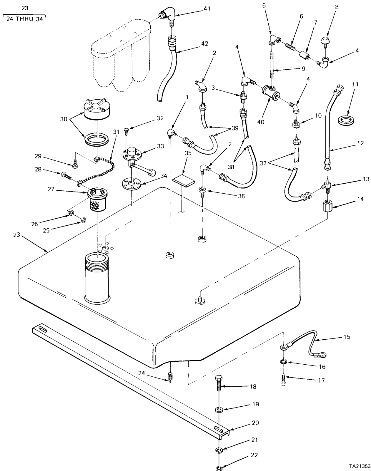
FIGURE 42. FUEL TANK (MODEL 2385 CRANE).
