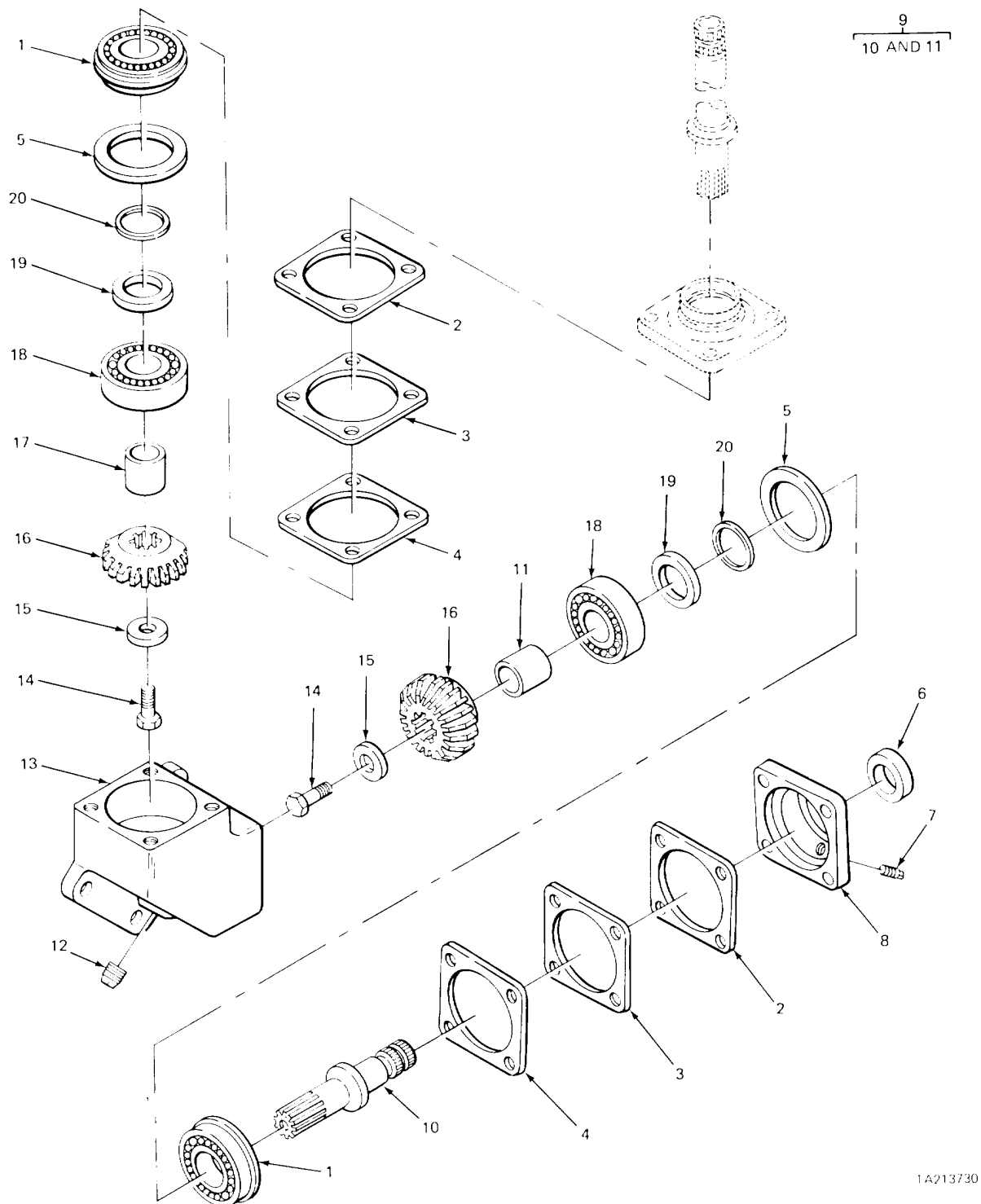
FIGURE 168. RIGHT ANGLE GEAR BOX FROM STEERING COLUMN (CARRIER)
