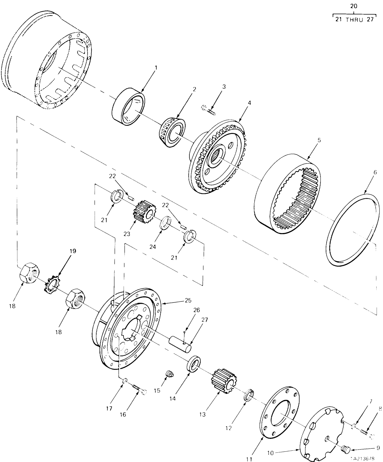
FIGURE 130. FRONT AXLE STEERING PARTS (CARRIER).
