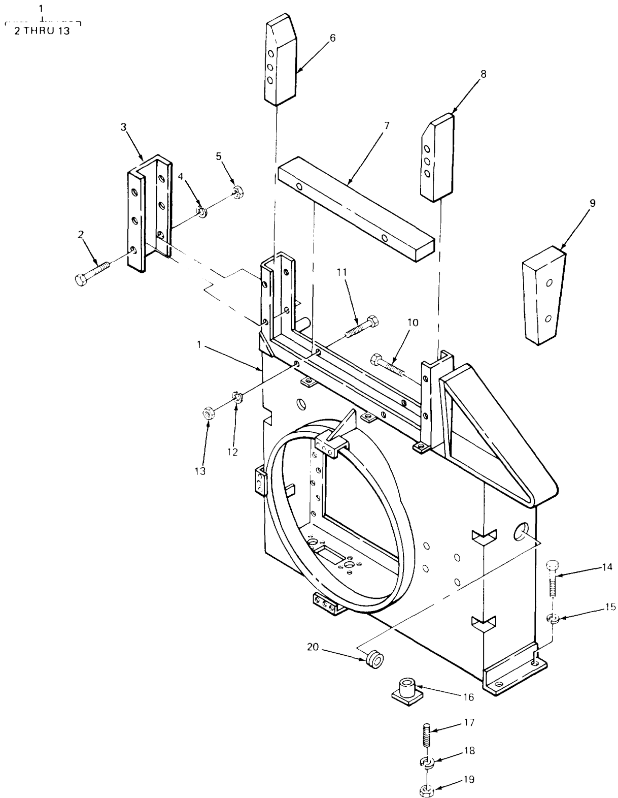
Figure 57. Rad1at0r Shr0ud and M0unt (M0del 2380 0arr1er)
