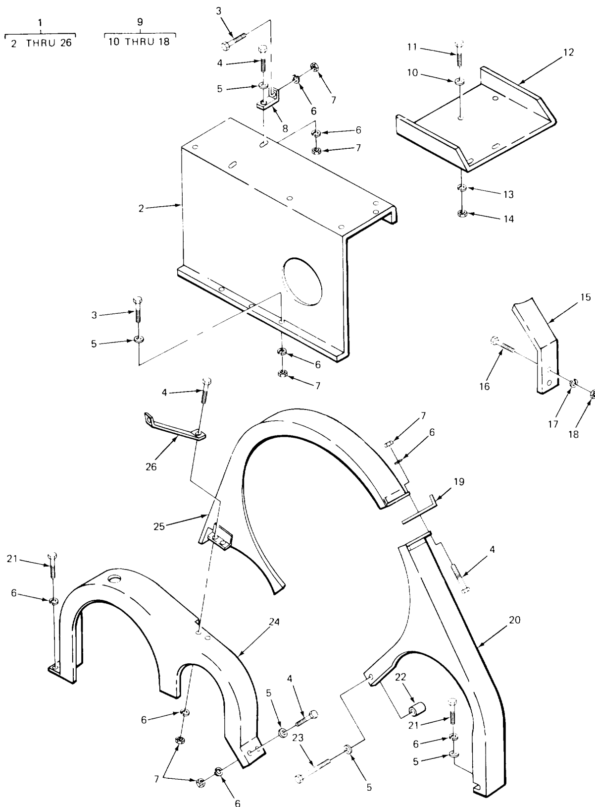
FIGURE 282. GEAR GAURD (CRANE).
