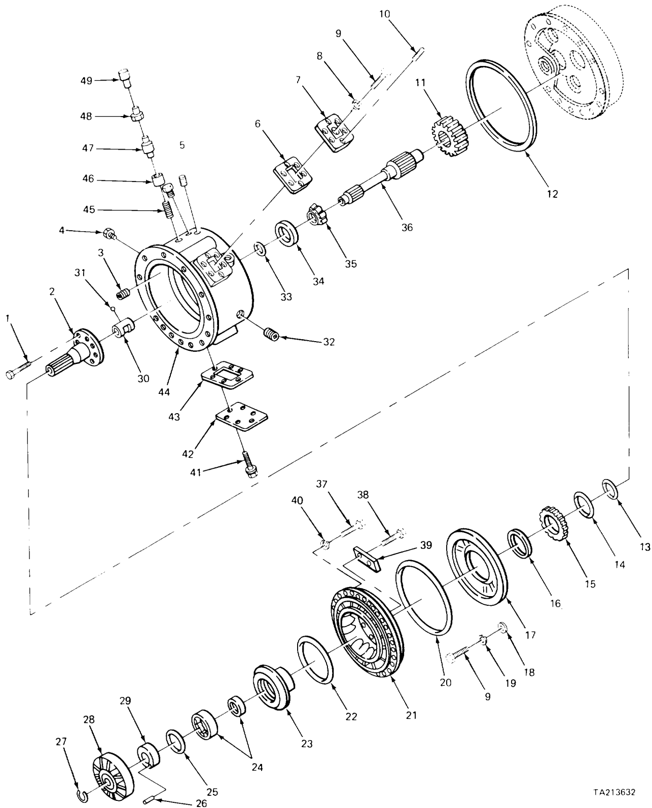
FIGURE 112. TORQUE CONVERTER COMPONENT PARTS AND BREATHER (CARRIER)
