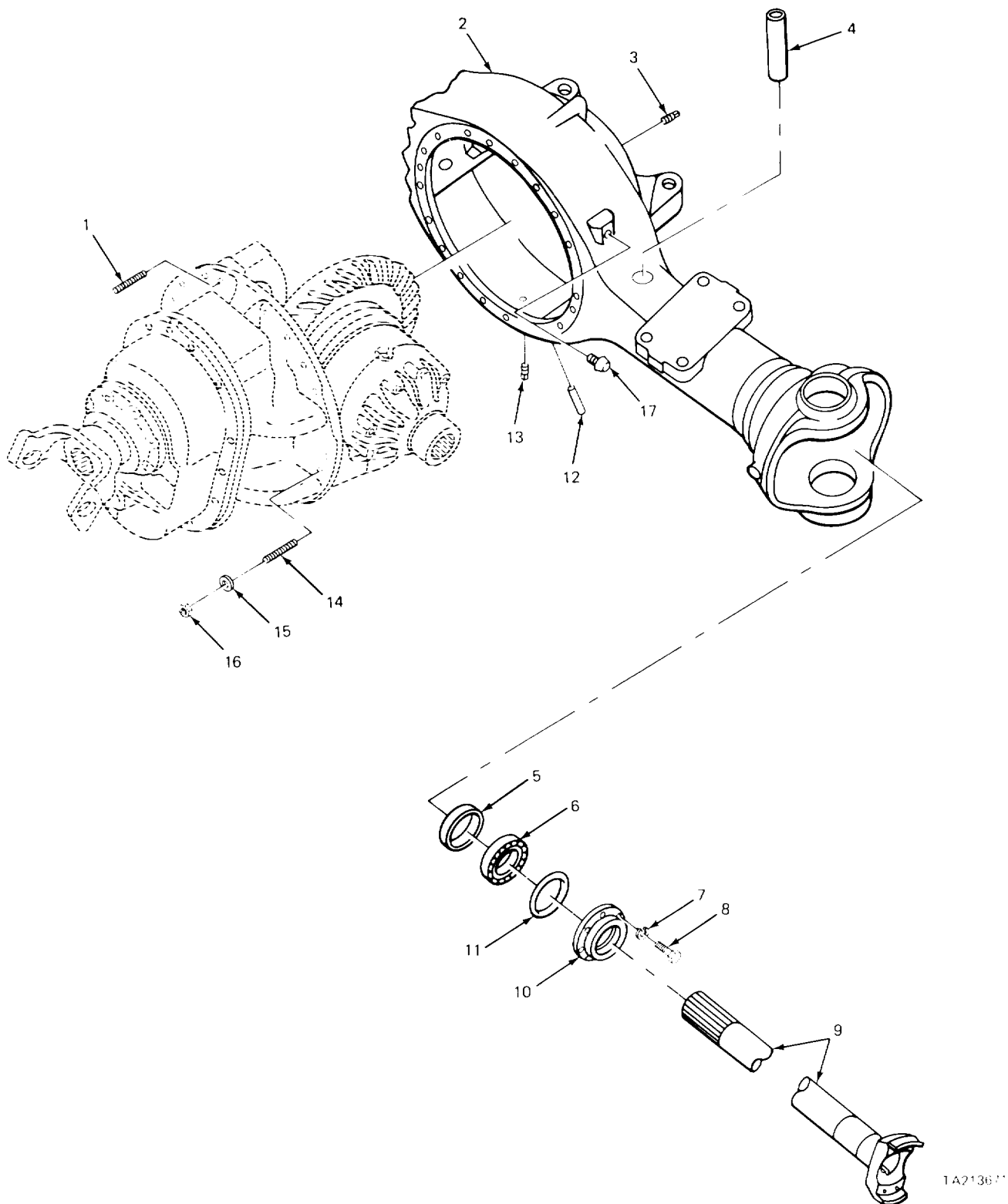
FIGURE 128. FRONT AXLE SHAFT AND HOUSING (CARRIER).
