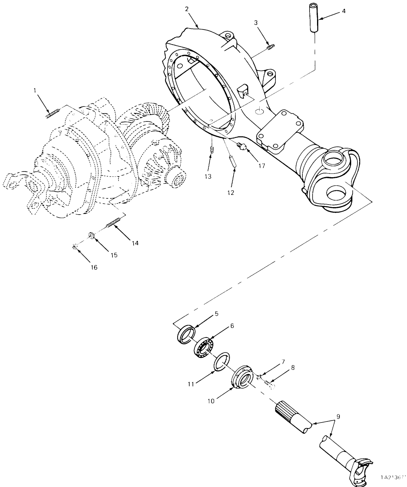
FIGURE 129. FRONT AXLE PLANETARY AND FINAL DRIVE (CARRIER).
