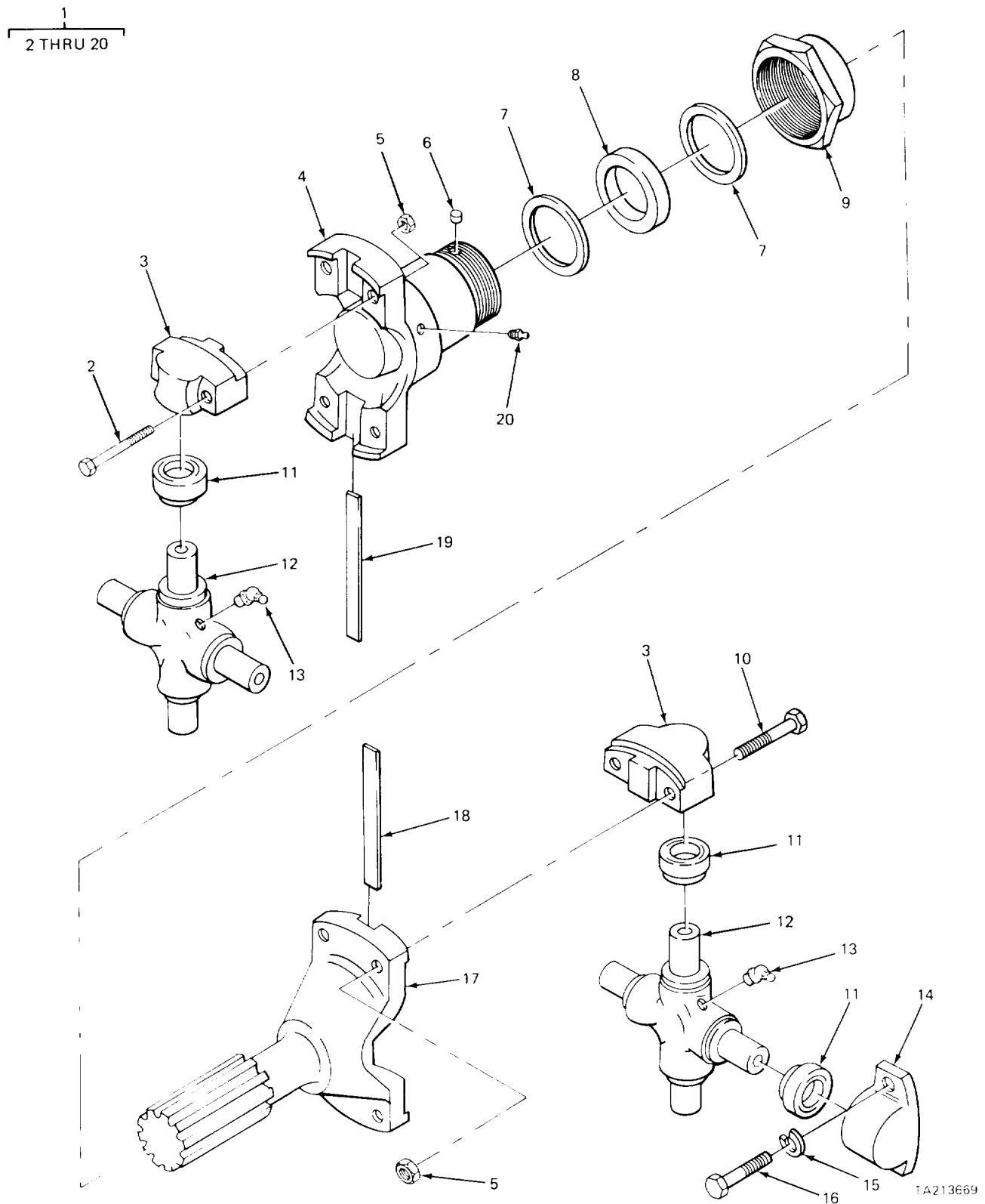
Figure 126. Propeller Shaft Transmission to Rear Axle.
