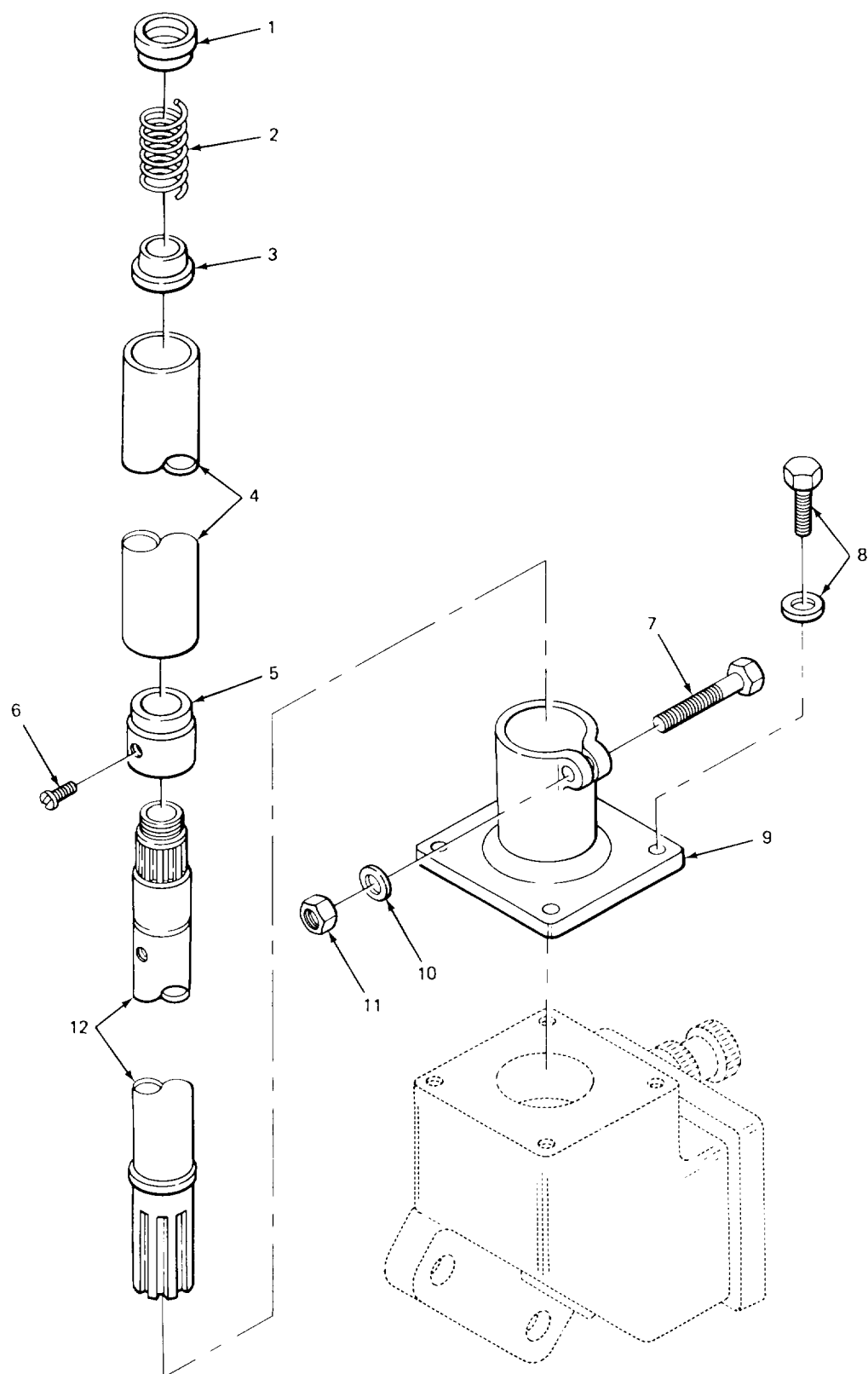
FIGURE 163. STEERING COLUMN (CARRIER)
