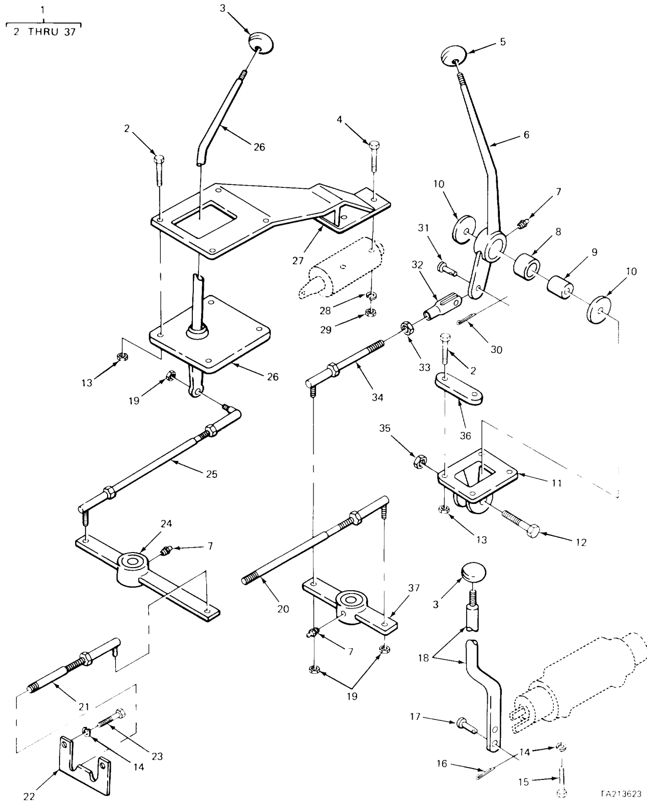
FIGURE 109. TRANSMISSION CONTROL LEVER ASSEMBLY (MODEL 2380 CARRIER)
