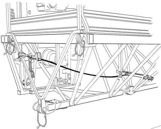
Platform section for around corner installations
